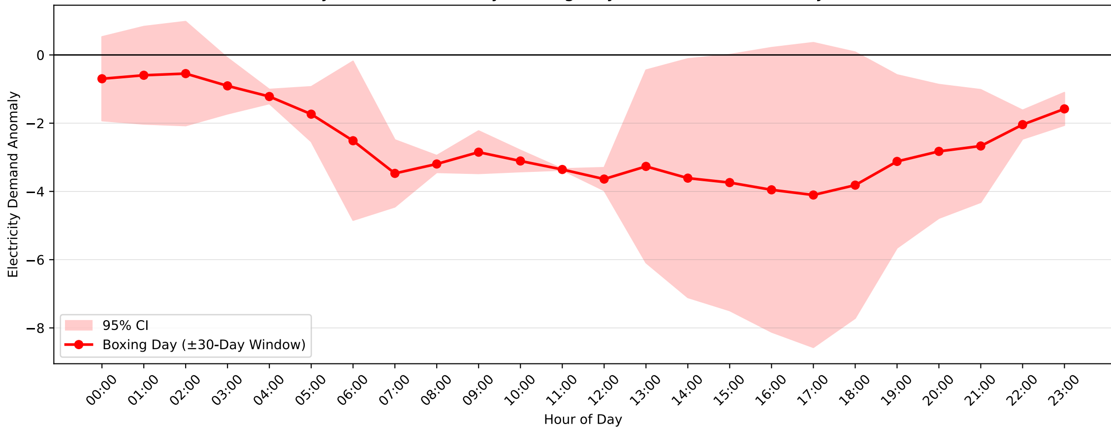
Revesby Demand Anomaly: Boxing Day (2013–2014, \pm 30 -Day Window)
