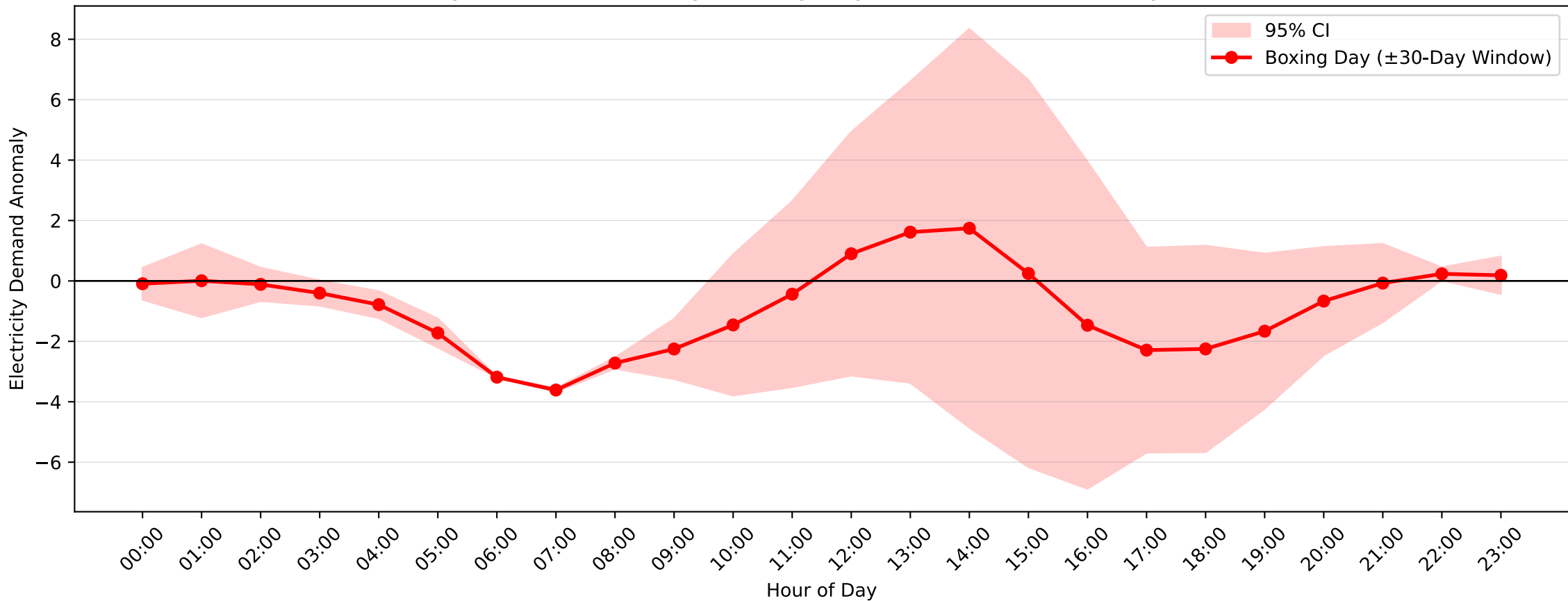
Revesby Demand Anomaly: Boxing Day (2015–2016, \pm 30 -Day Window)
