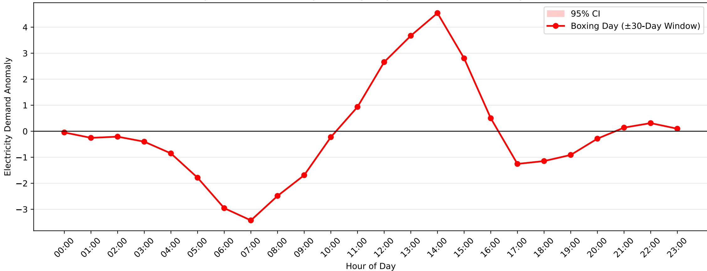
Revesby Demand Anomaly: Boxing Day (2016–2017, \pm 30 -Day Window)
