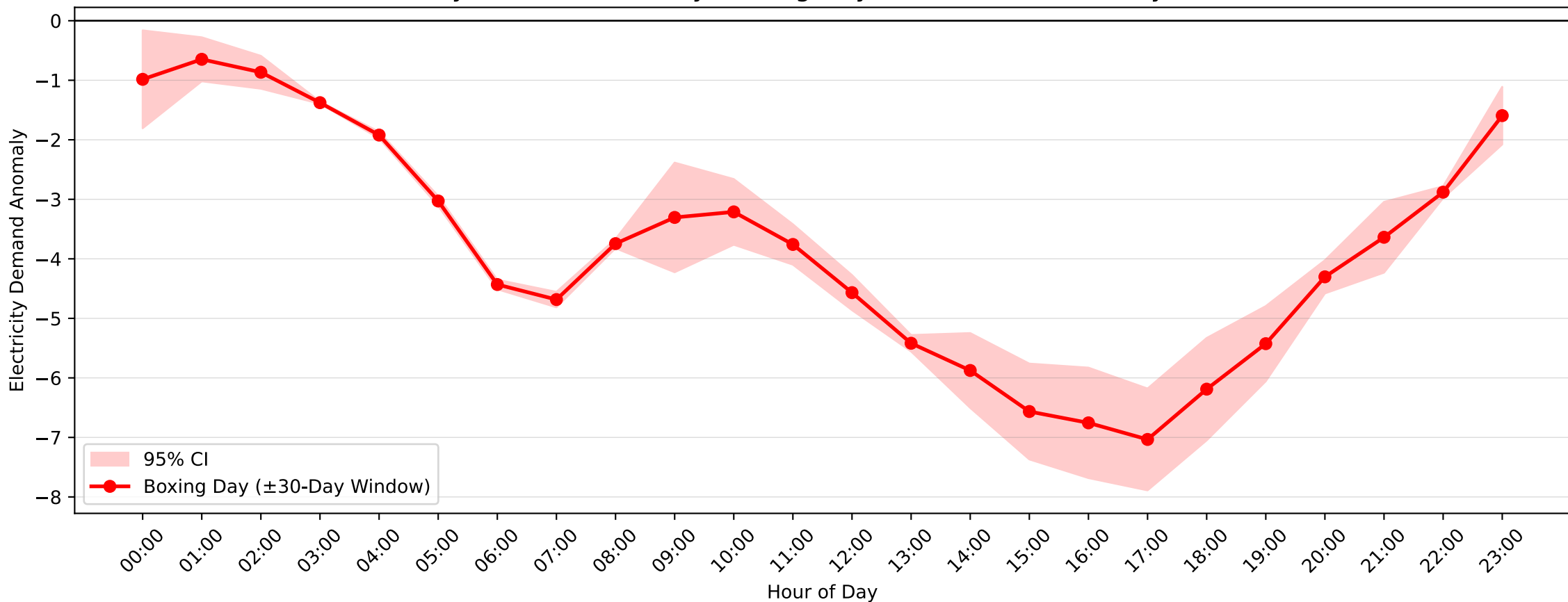
Revesby Demand Anomaly: Boxing Day (2006–2007, \pm 30 -Day Window)
