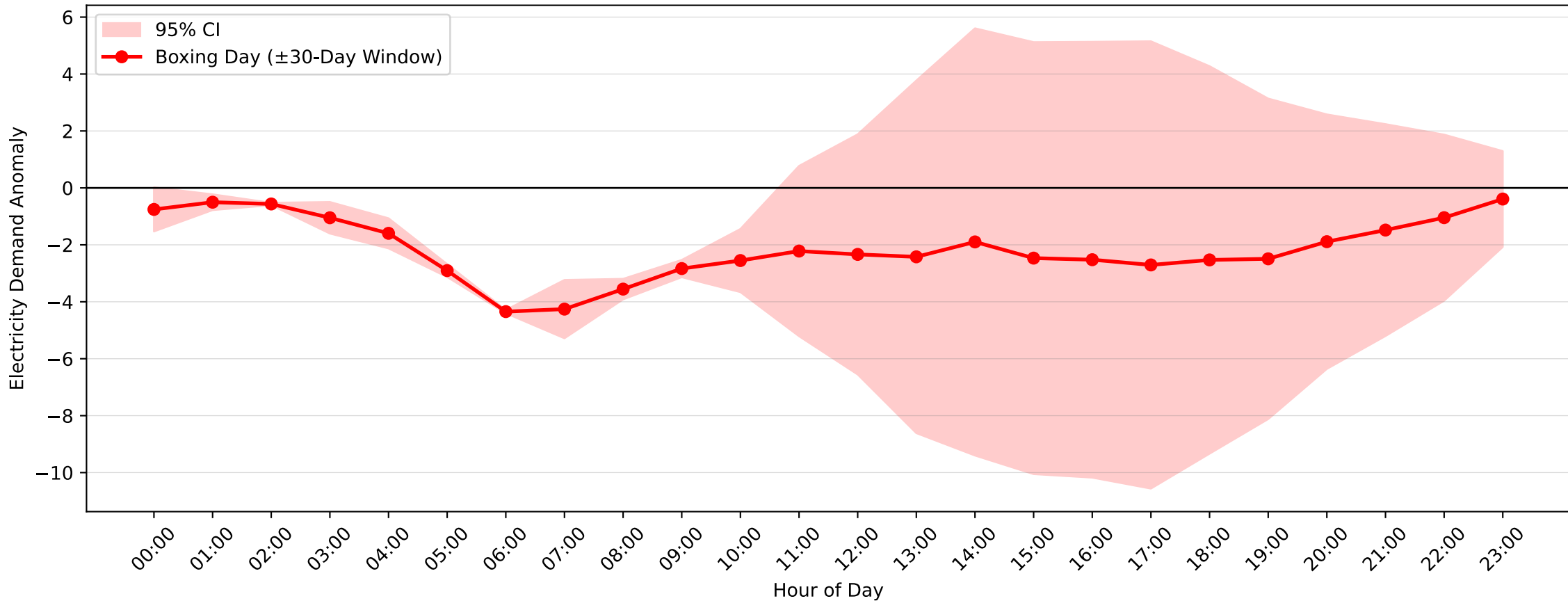
Revesby Demand Anomaly: Boxing Day (2007-2008, \pm 30 -Day Window)
