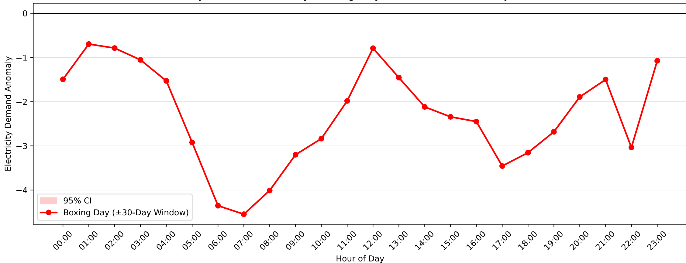
Revesby Demand Anomaly: Boxing Day (2004–2005, \pm 30 -Day Window)
